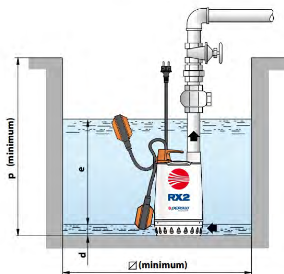
Typical installation
