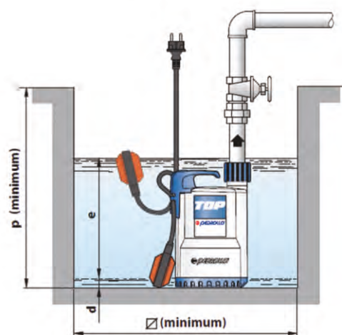
Typical installation
