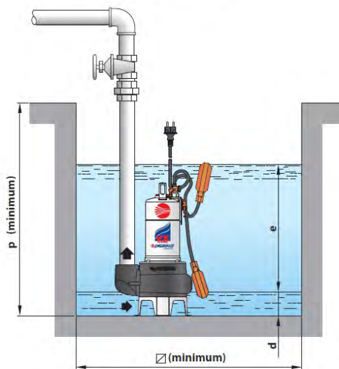
Typical installation
