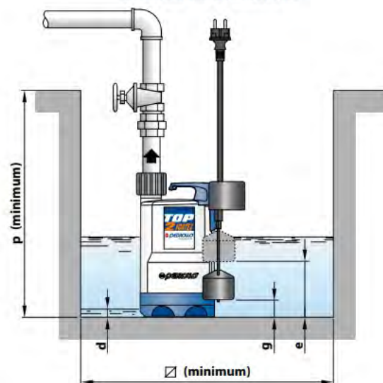
Standard installation
