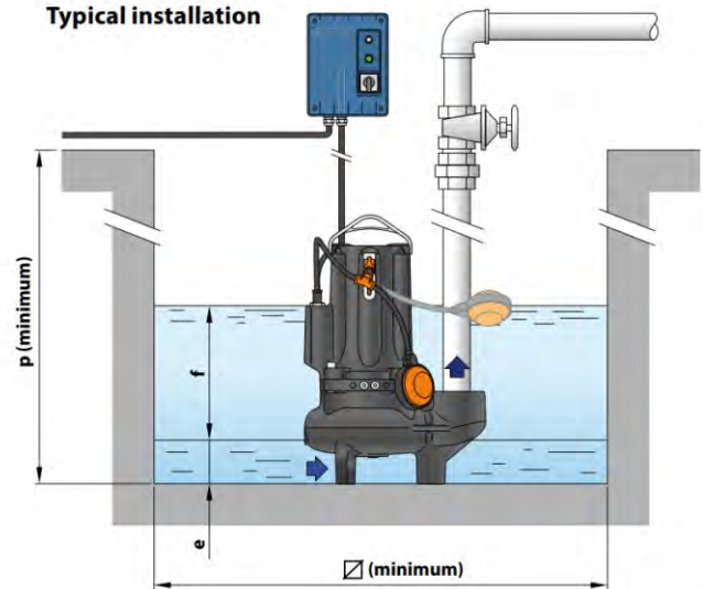
Typical installation
