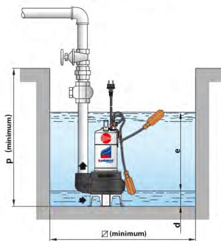
Typical installation
