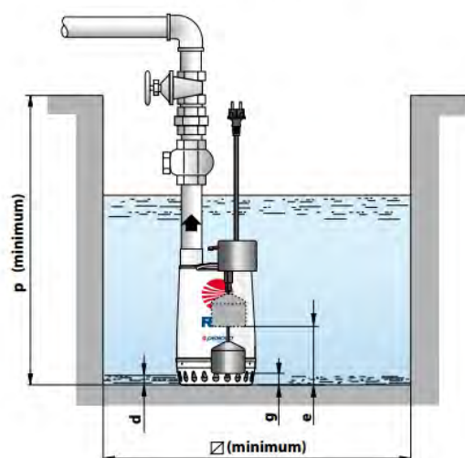
Typical installation
