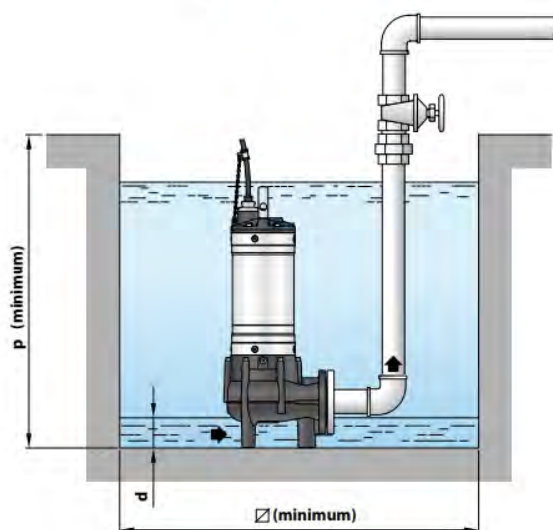
Standard installation
