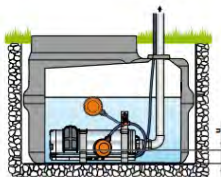
Horizontal installation
